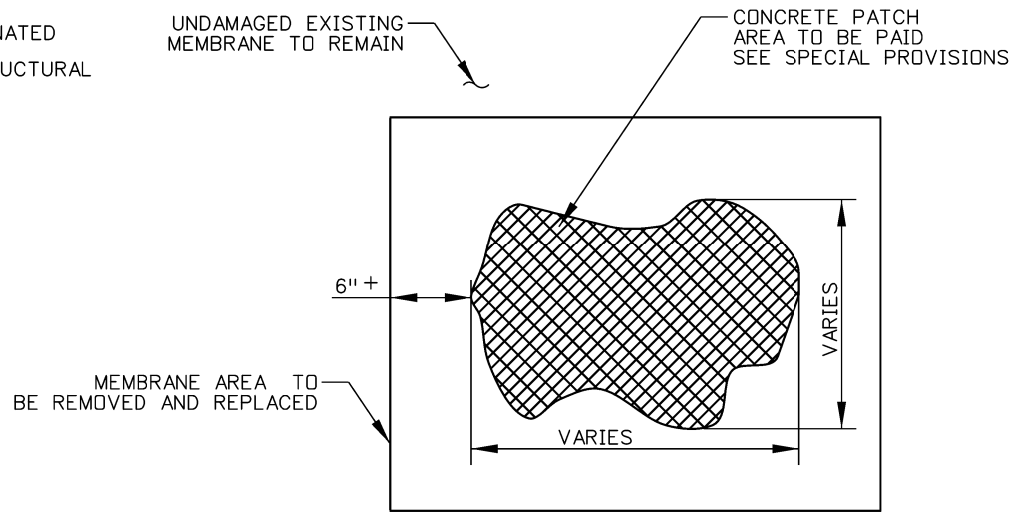
CONCRETE PATCHING PLAN N.T.S.
