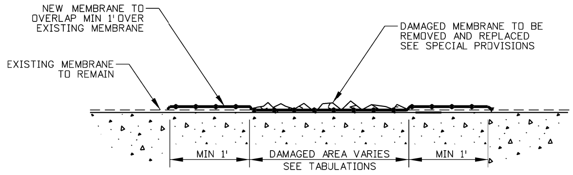
WATERPROOFING MEMBRANE PATCH SECTION N.T.S.
