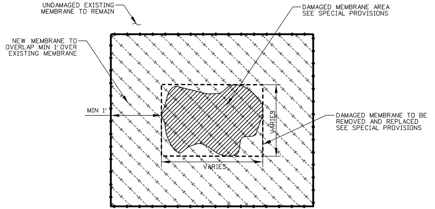
WATERPROOFING MEMBRANE PATCH PLAN N.T.S.
