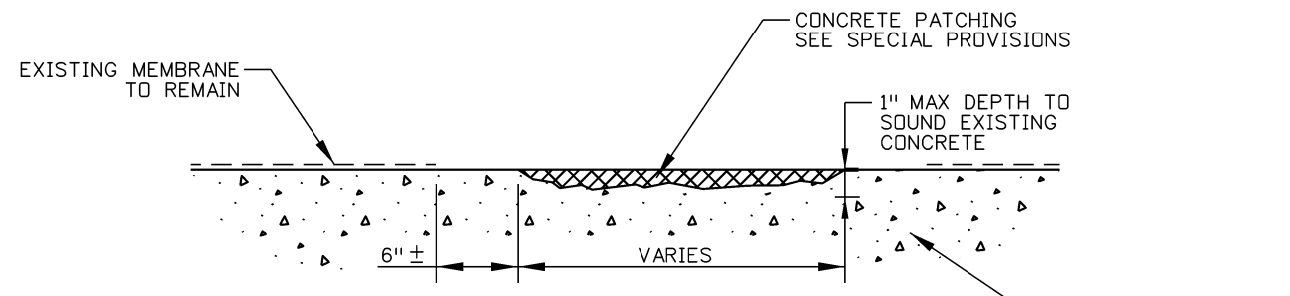
EISENHOWER TUNNEL CONCRETE PATCHING SECTION N.T.S.
